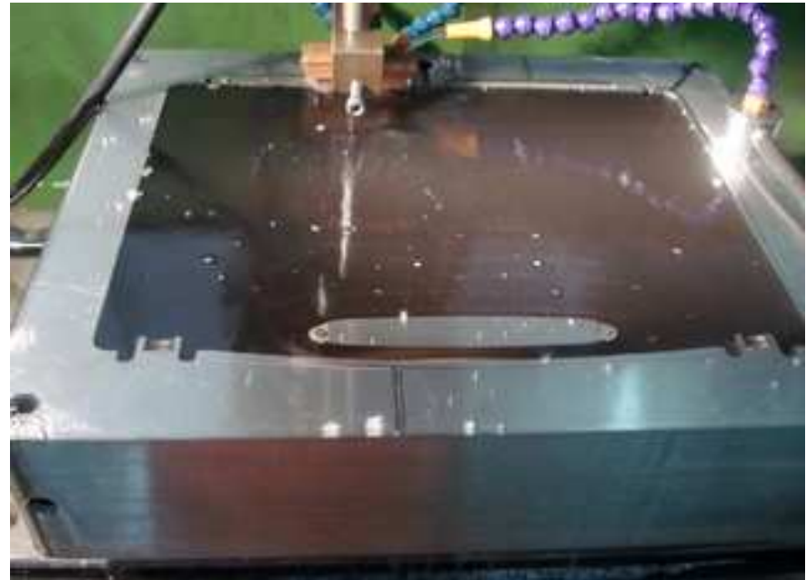
Spark eroding
